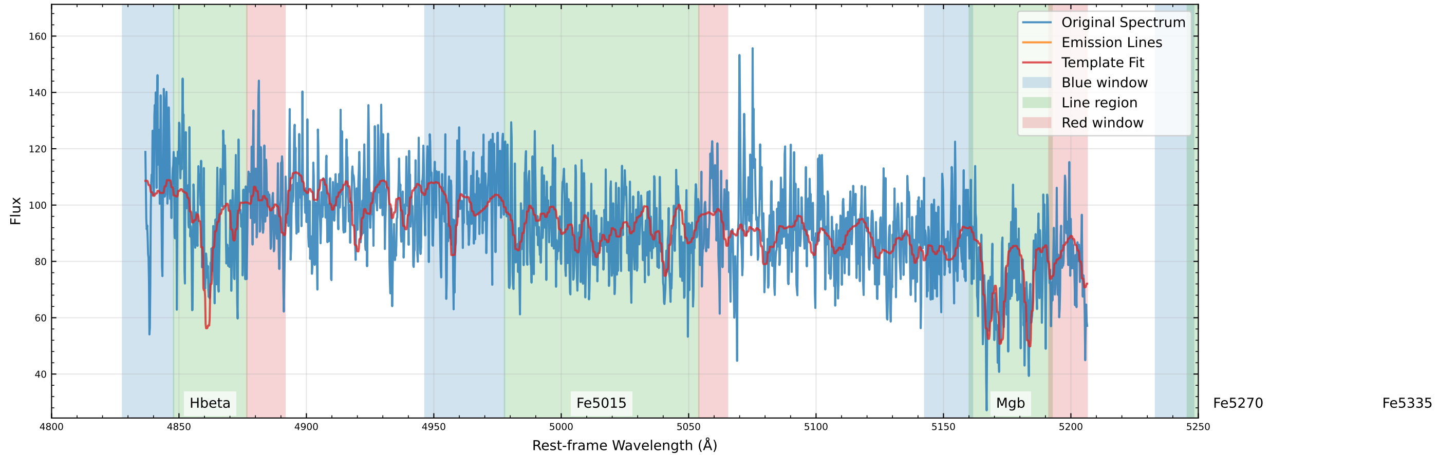
Original Data Comparison (v_star=-20.3 km/s, v_gas=-145.5 km/s)
