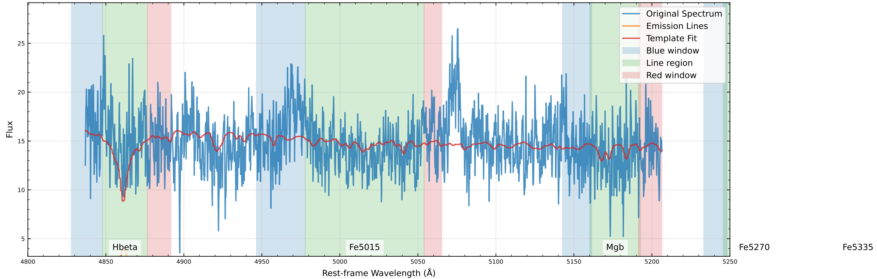
Original Data Comparison (v_star=129.9 km/s, v_gas=147.8 km/s)
