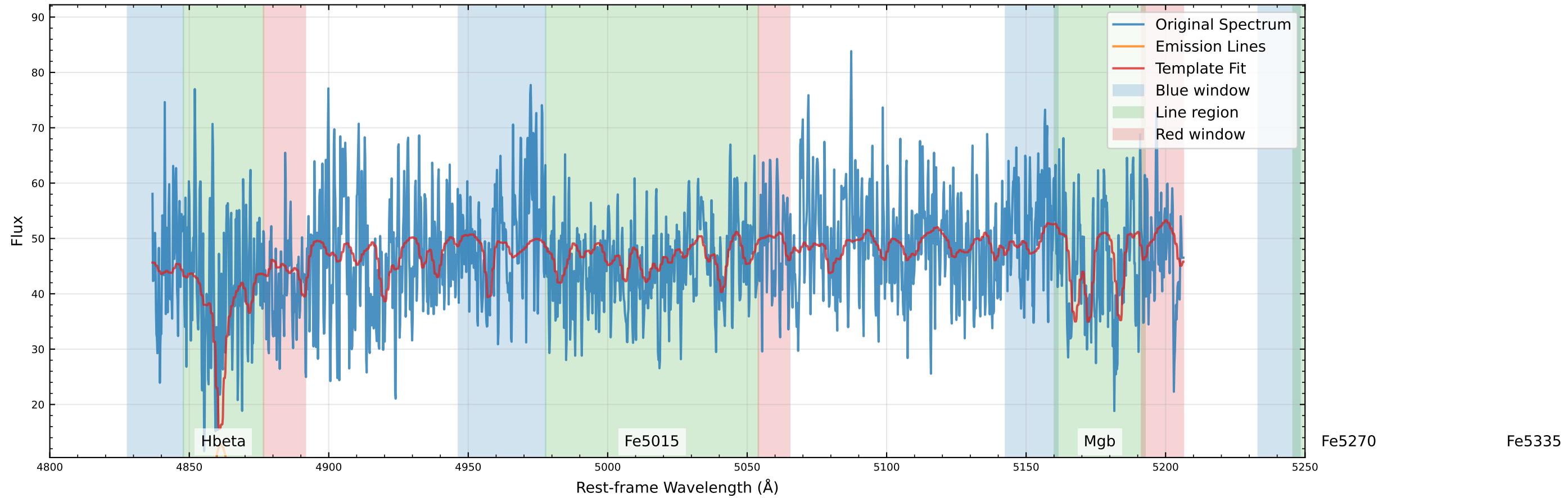
Original Data Comparison (v_star=-76.3 km/s, v_gas=-55.2 km/s)
