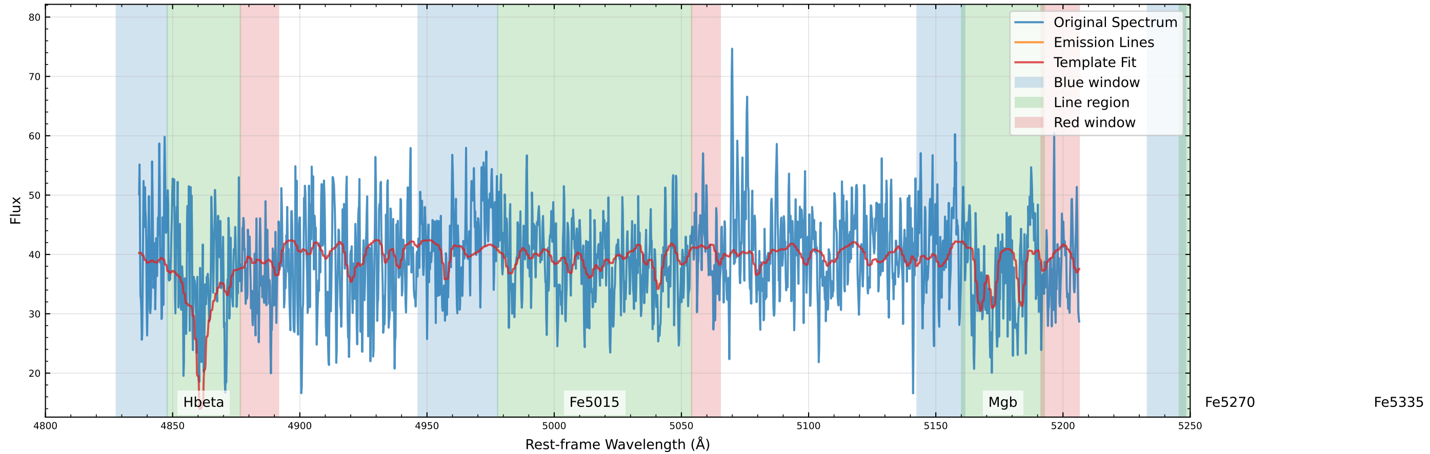
Original Data Comparison (v_star=-29.4 km/s, v_gas=-73.6 km/s)
