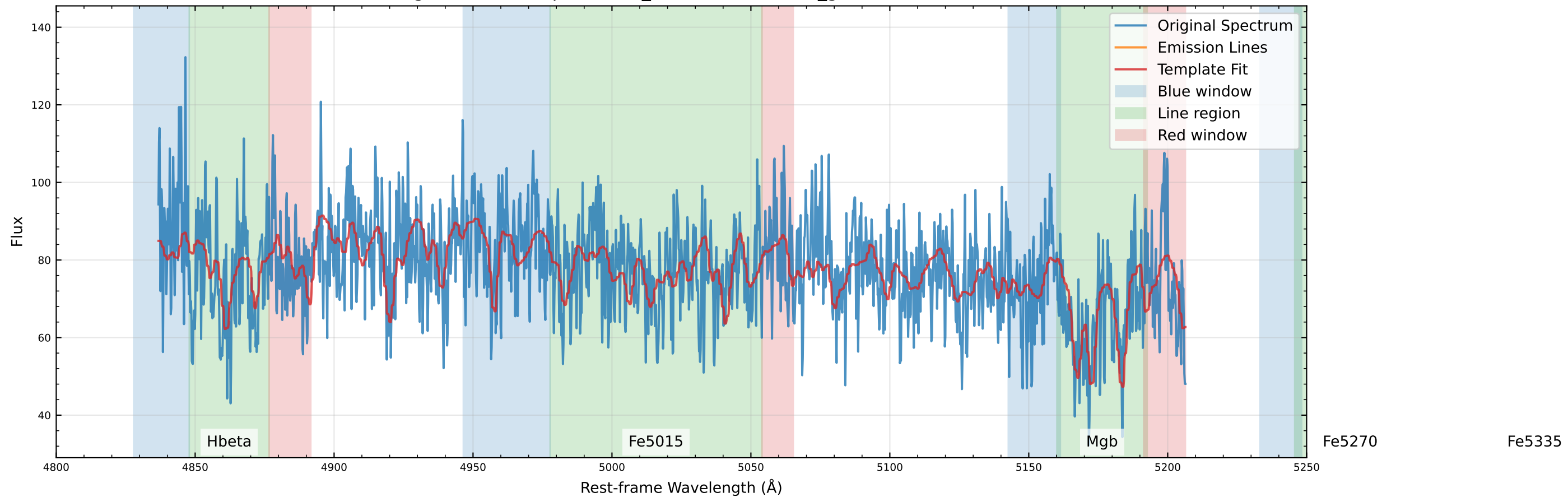
Original Data Comparison (v_star=-39.9 km/s, v_gas=-33.9 km/s)
