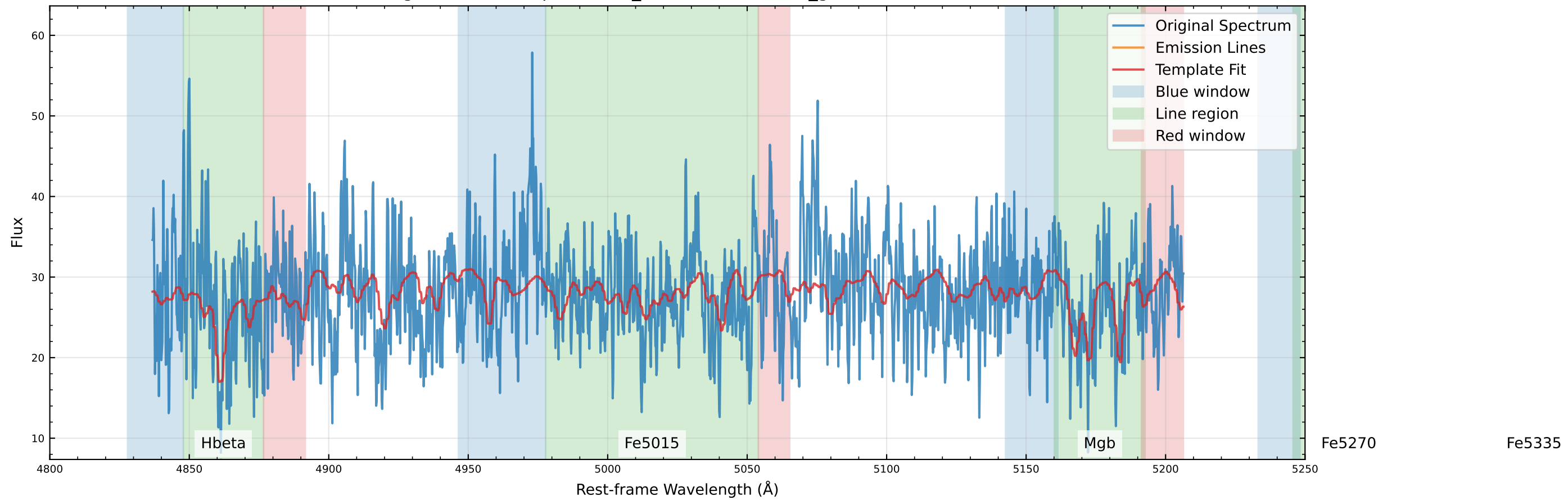
Original Data Comparison (v_star=-55.3 km/s, v_gas=-310.6 km/s)
