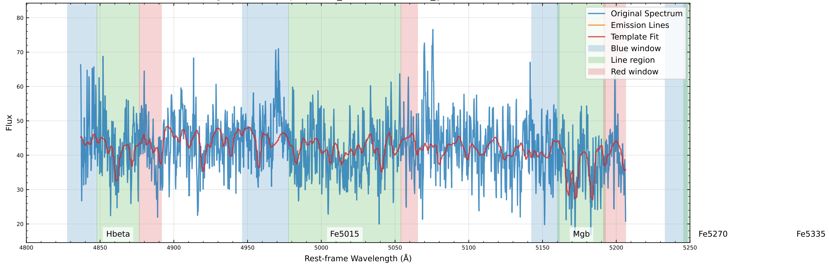
Original Data Comparison (v_star=-12.7 km/s, v_gas=-16.4 km/s)
