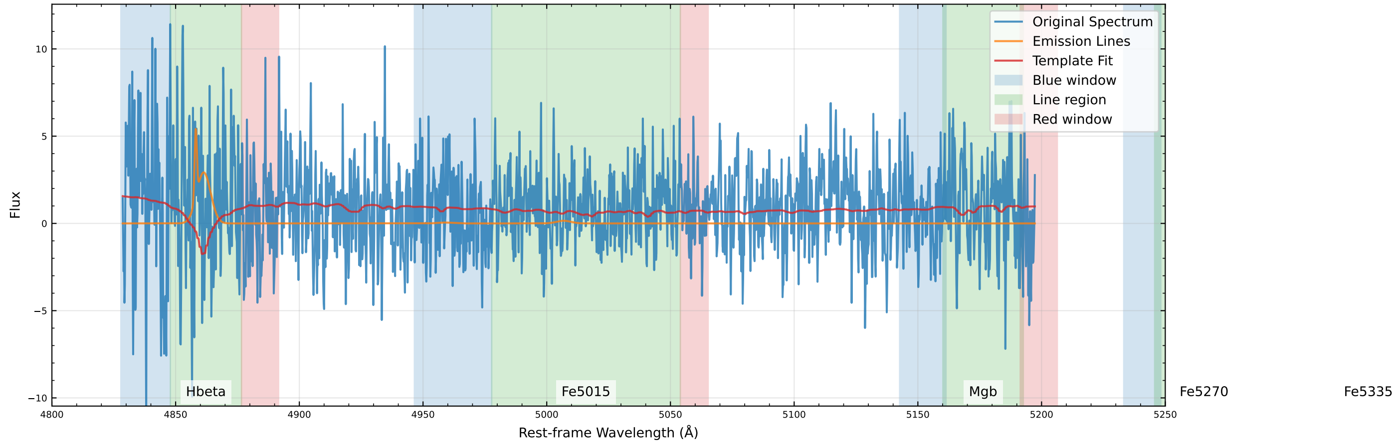
Original Data Comparison (v_star=362.7 km/s, v_gas=539.0 km/s)
