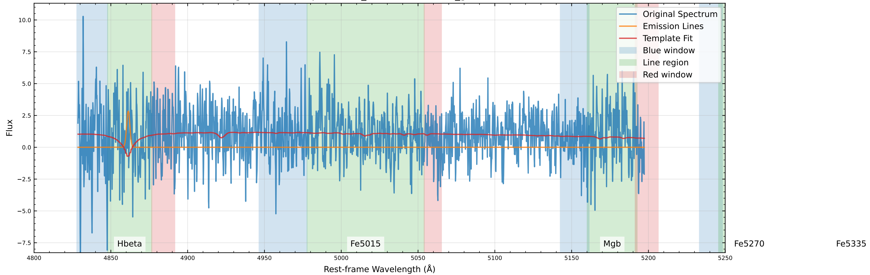
Original Data Comparison (v_star=11.9 km/s, v_gas=81.5 km/s)
