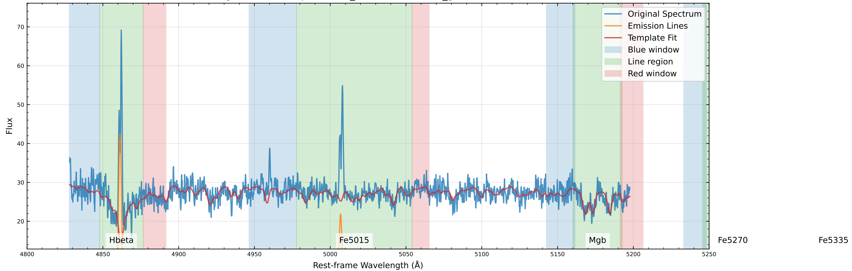
Original Data Comparison (v_star=47.0 km/s, v_gas=35.5 km/s)
