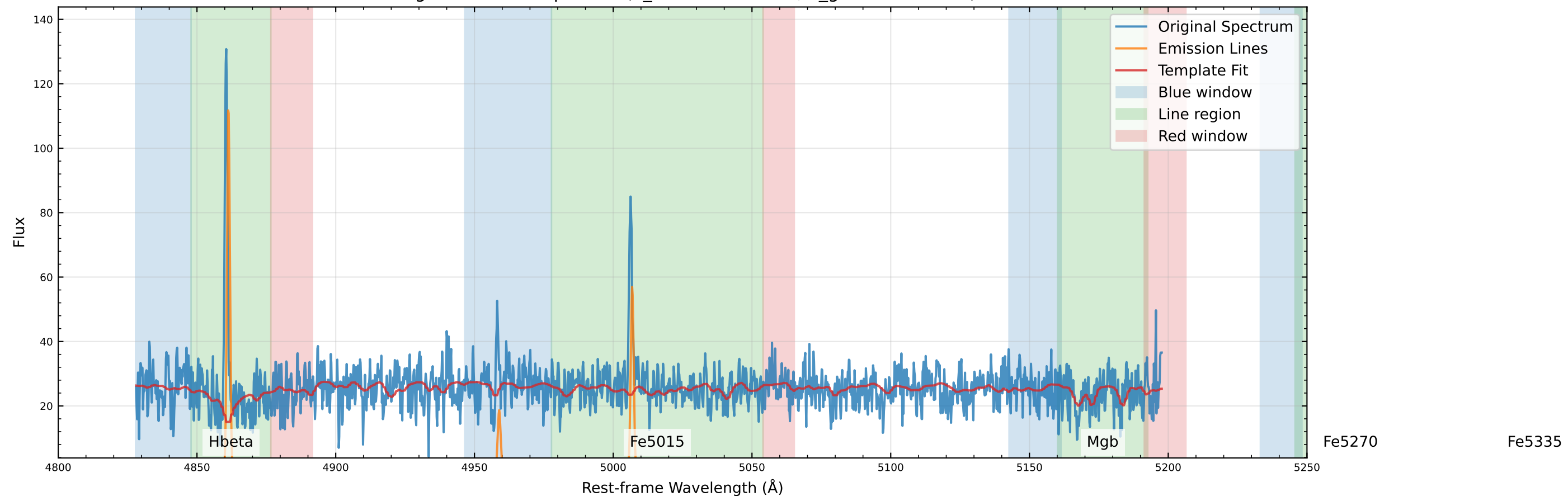
Original Data Comparison (v_star=-53.1 km/s, v_gas=-47.1 km/s)
