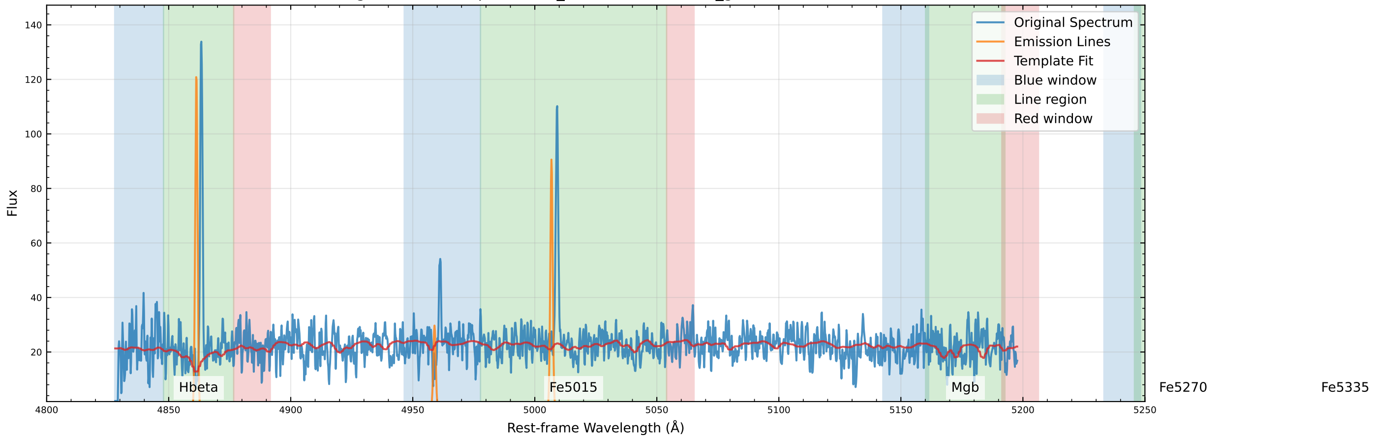
Original Data Comparison (v_star=140.6 km/s, v_gas=129.2 km/s)
