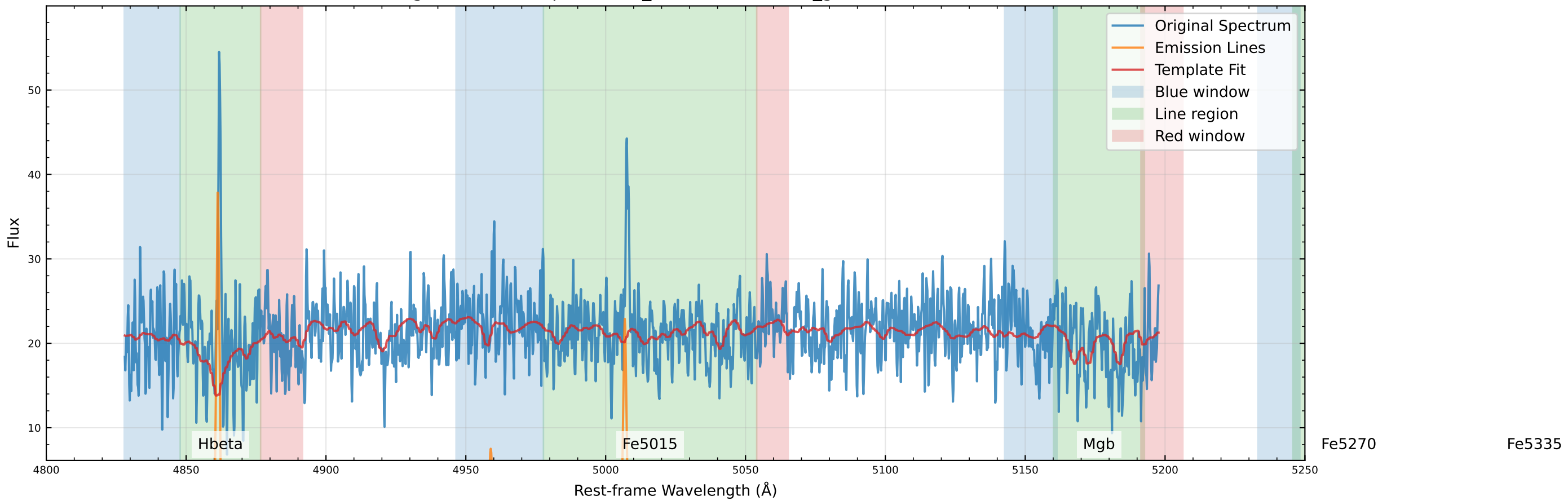
Original Data Comparison (v_star=34.3 km/s, v_gas=40.4 km/s)
