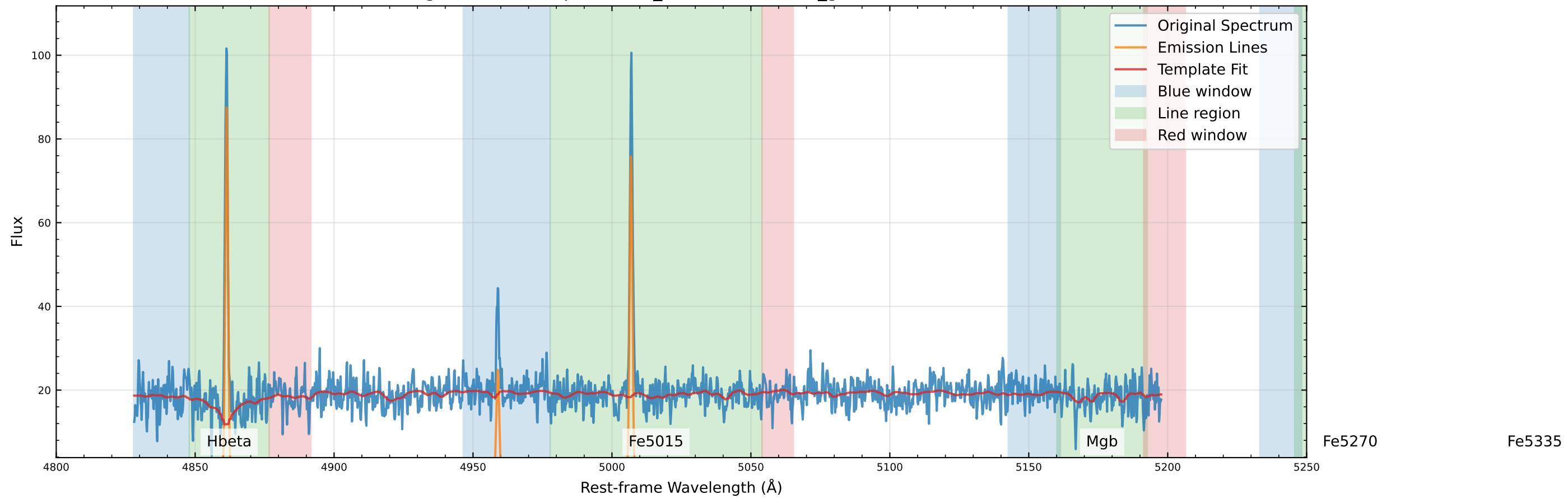
Original Data Comparison (v_star=-5.9 km/s, v_gas=-0.7 km/s)
