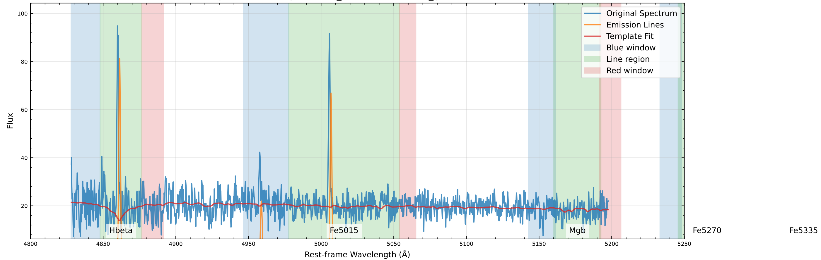
Original Data Comparison (v_star=-68.8 km/s, v_gas=-73.1 km/s)
