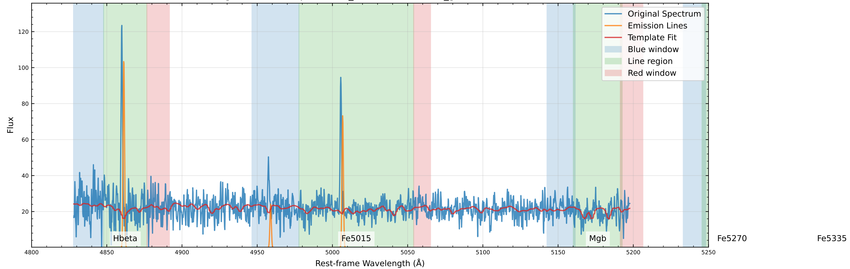
Original Data Comparison (v_star=-76.0 km/s, v_gas=-81.1 km/s)
