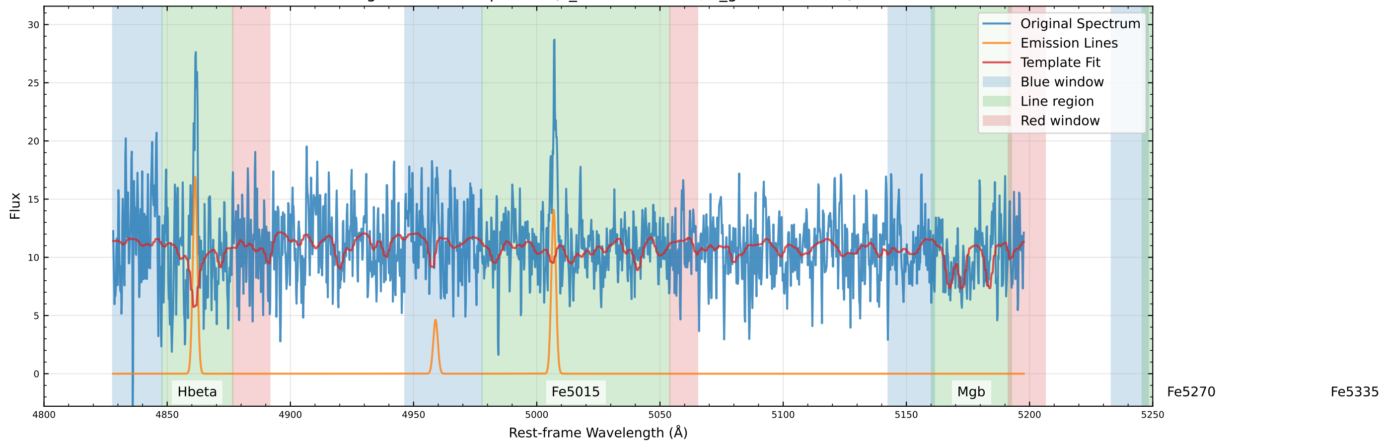
Original Data Comparison (v_star=17.0 km/s, v_gas=13.9 km/s)
