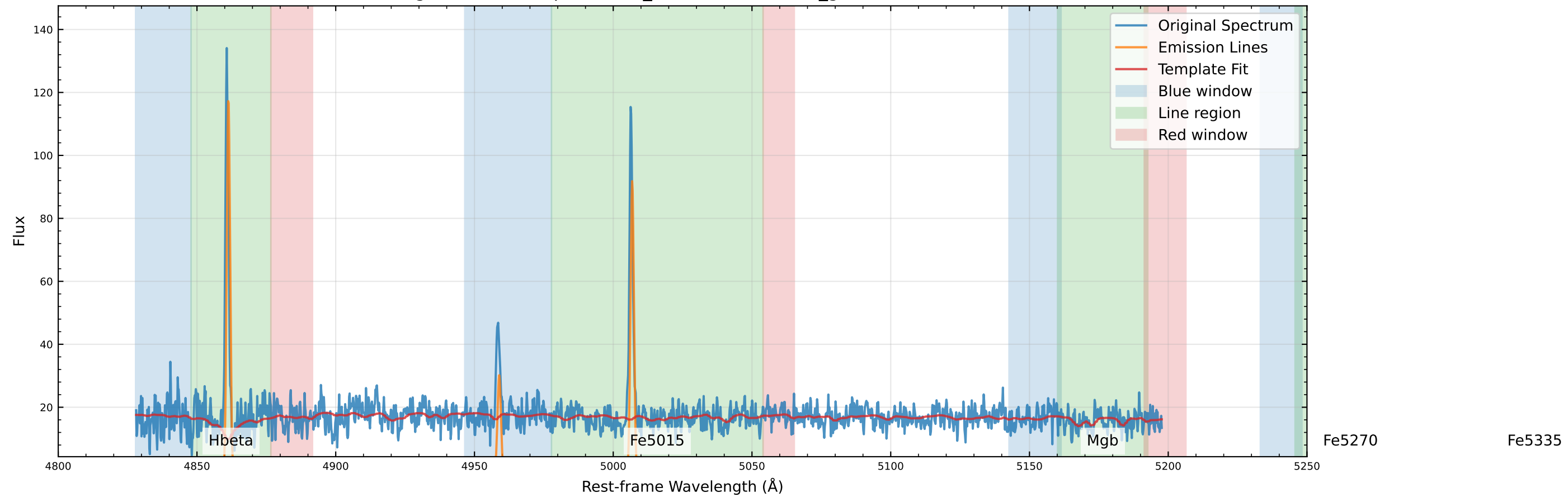
Original Data Comparison (v_star=-47.4 km/s, v_gas=-30.3 km/s)
