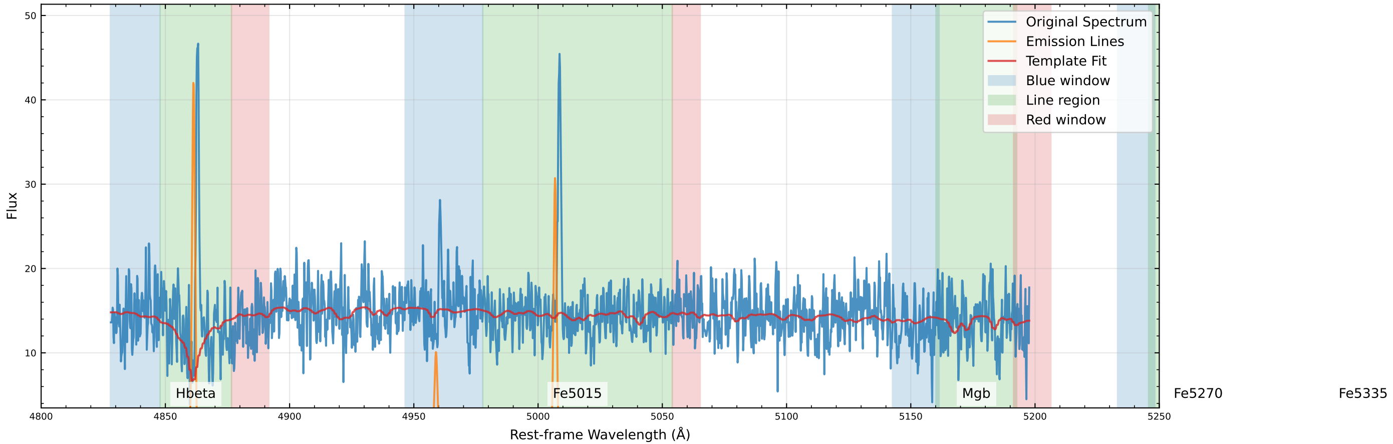
Original Data Comparison (v_star=107.5 km/s, v_gas=102.3 km/s)
