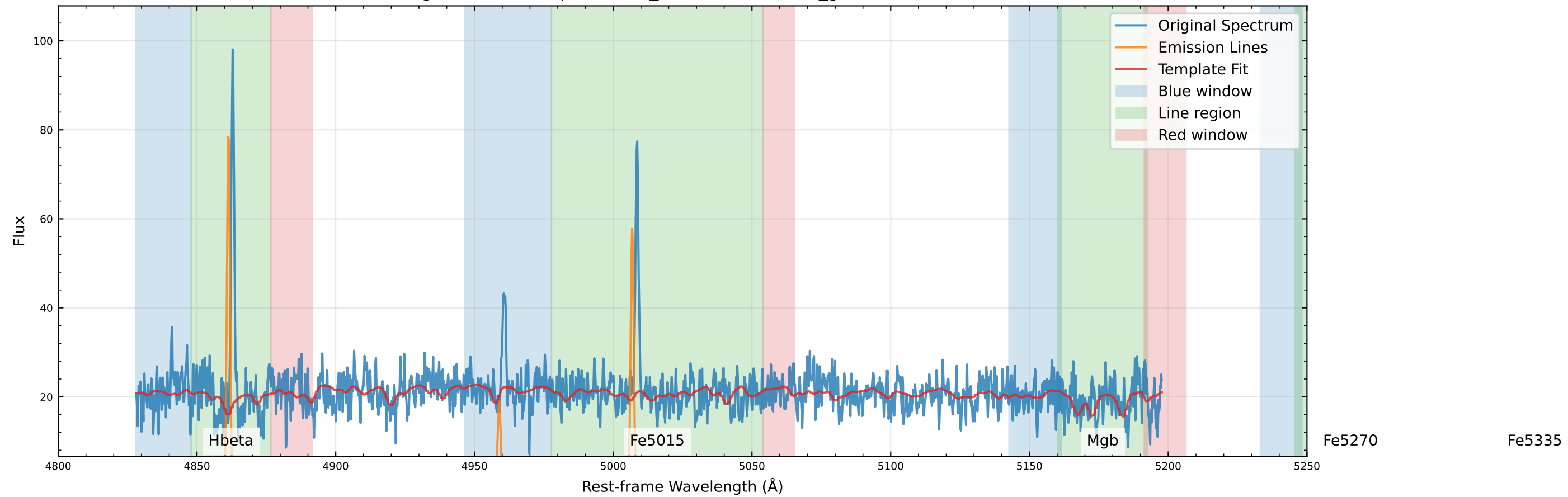
Original Data Comparison (v_star=87.6 km/s, v_gas=97.4 km/s)
