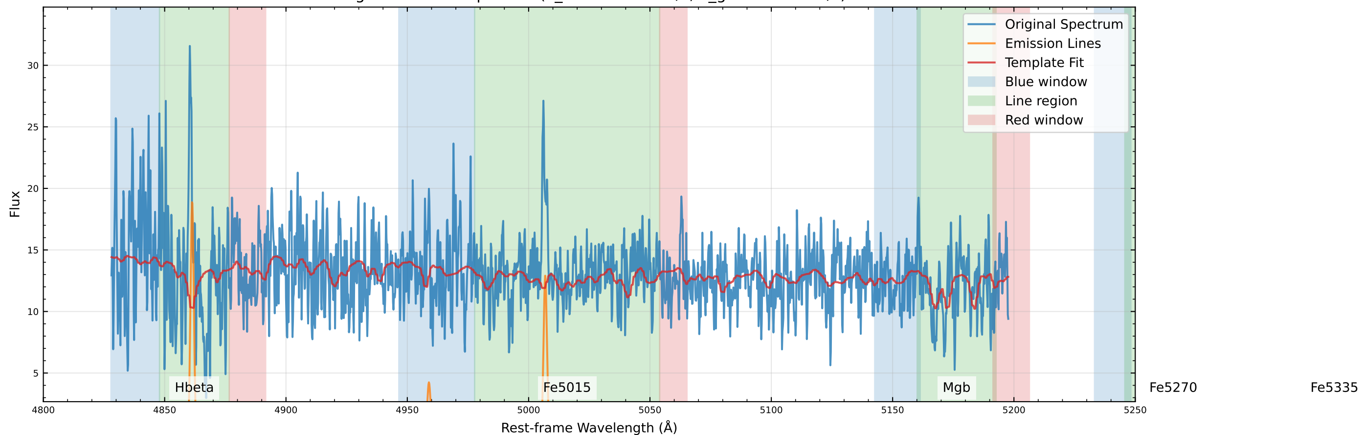
Original Data Comparison (v_star=-34.8 km/s, v_gas=-44.6 km/s)
