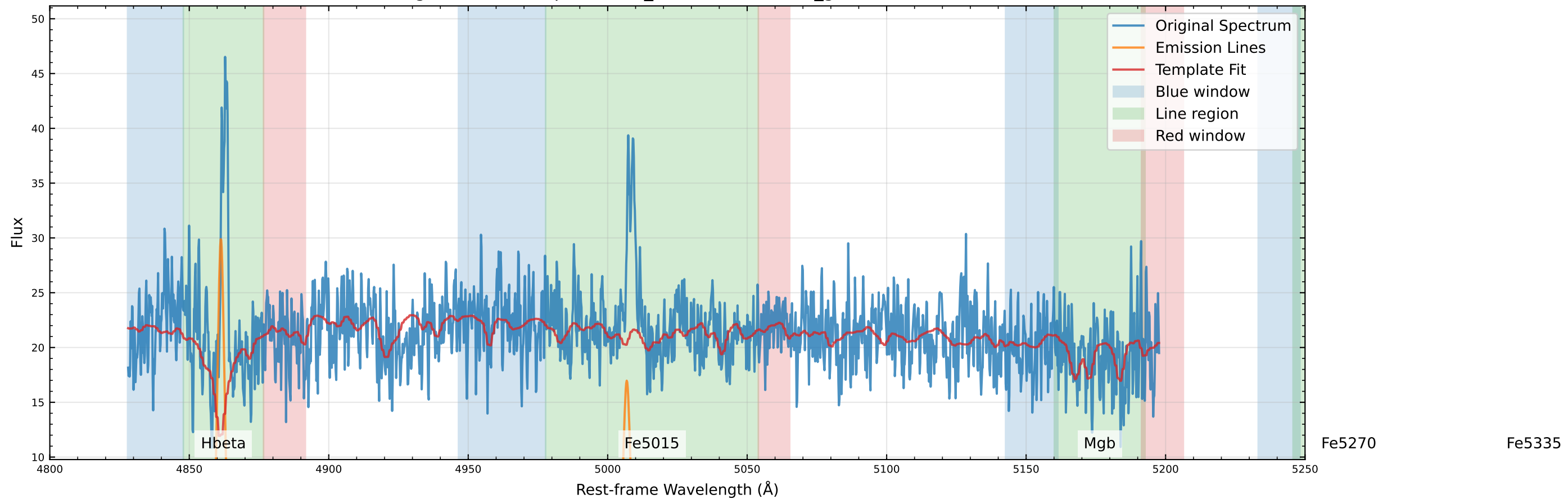
Original Data Comparison (v_star=45.3 km/s, v_gas=86.4 km/s)
