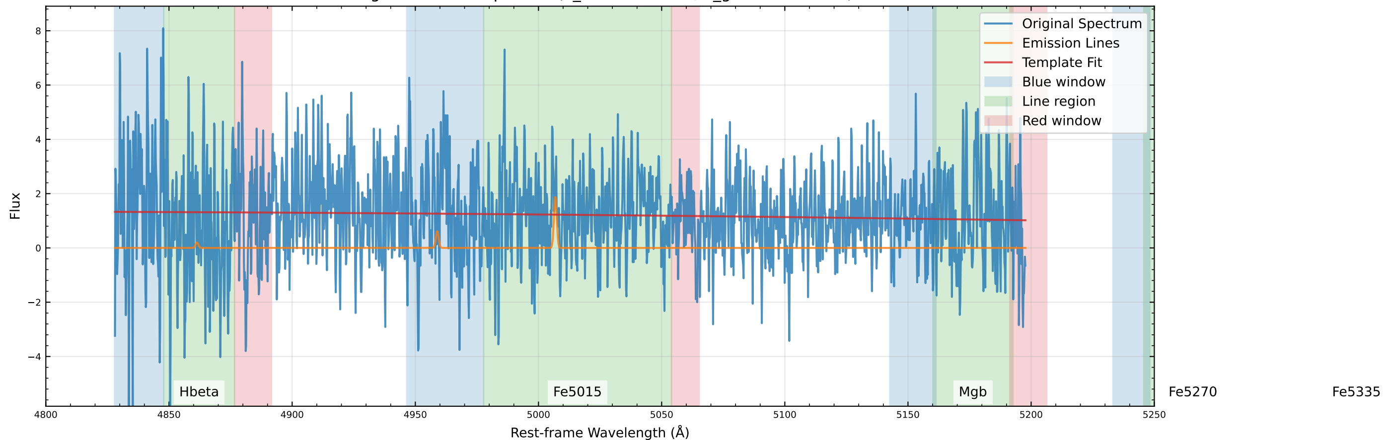
Original Data Comparison (v_star=0.0 km/s, v_gas=-56.9 km/s)
