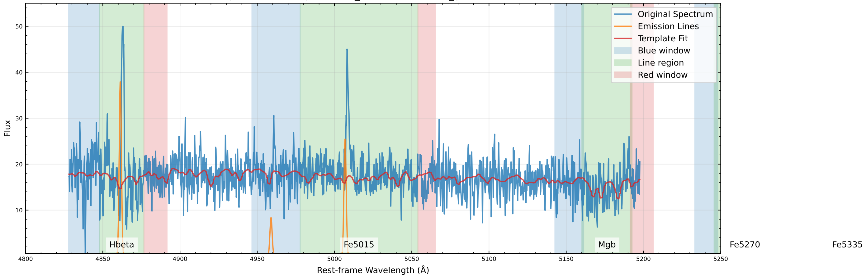
Original Data Comparison (v_star=13.8 km/s, v_gas=95.4 km/s)
