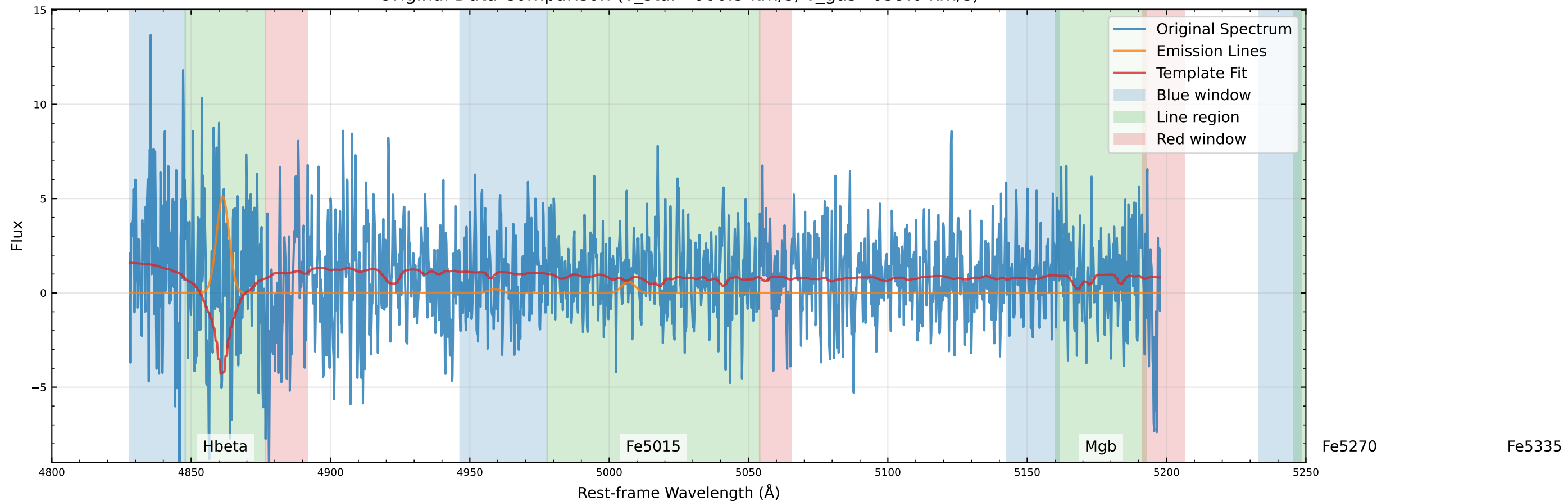
Original Data Comparison (v_star=666.3 km/s, v_gas=639.0 km/s)
