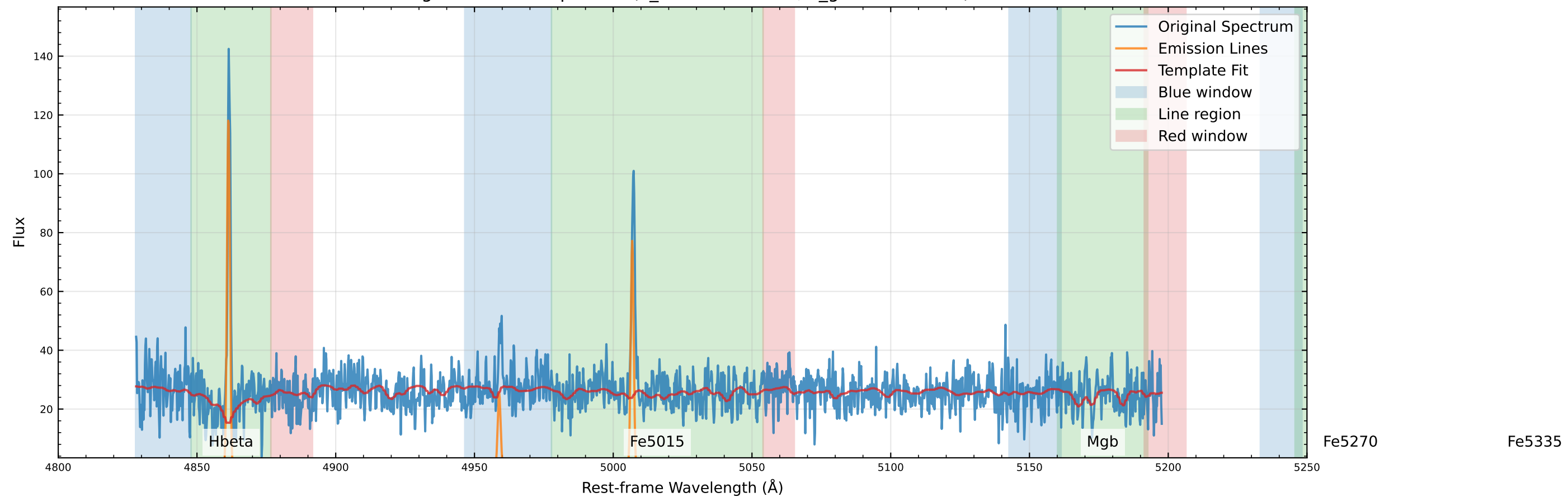
Original Data Comparison (v_star=17.1 km/s, v_gas=16.8 km/s)
