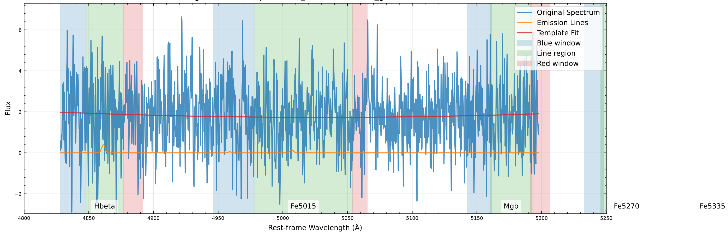
Original Data Comparison (v_star=0.0 km/s, v_gas=-13.6 km/s)
