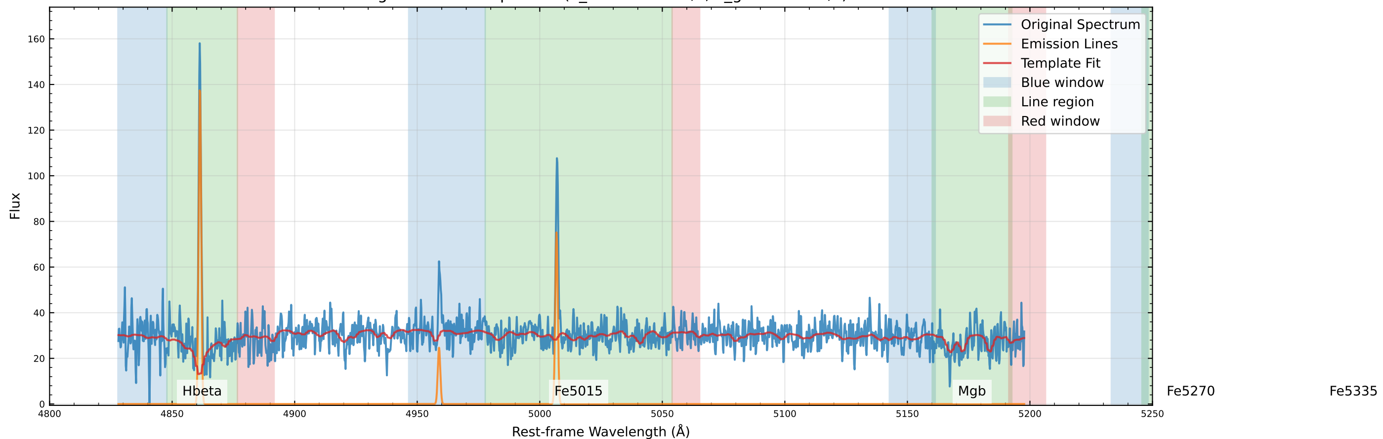
Original Data Comparison ( v_{\text{star}}=-9.4 km/s, v_{\text{gas}}=2.7 km/s)
