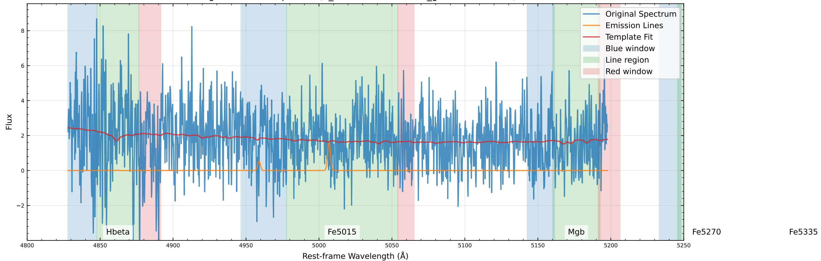
Original Data Comparison (v_star=-210.0 km/s, v_gas=-274.5 km/s)
