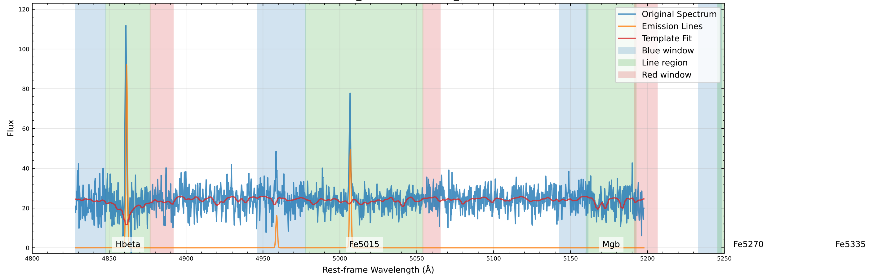
Original Data Comparison (v_star=-20.1 km/s, v_gas=-28.2 km/s)
