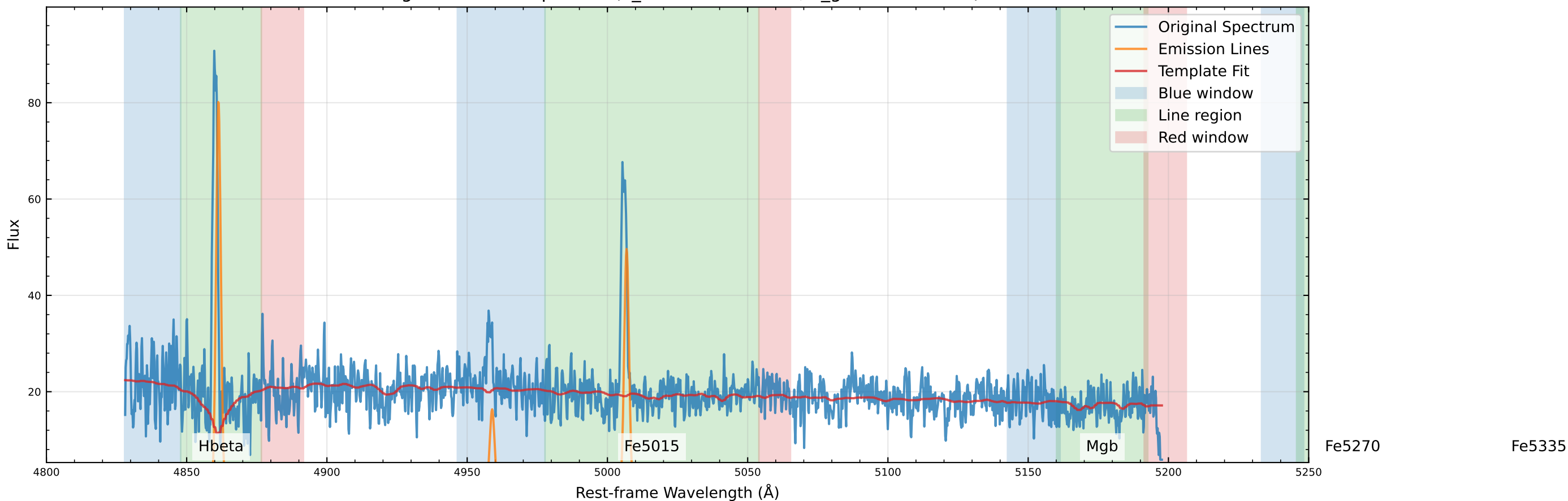
Original Data Comparison (v_star=-106.0 km/s, v_gas=-69.8 km/s)
