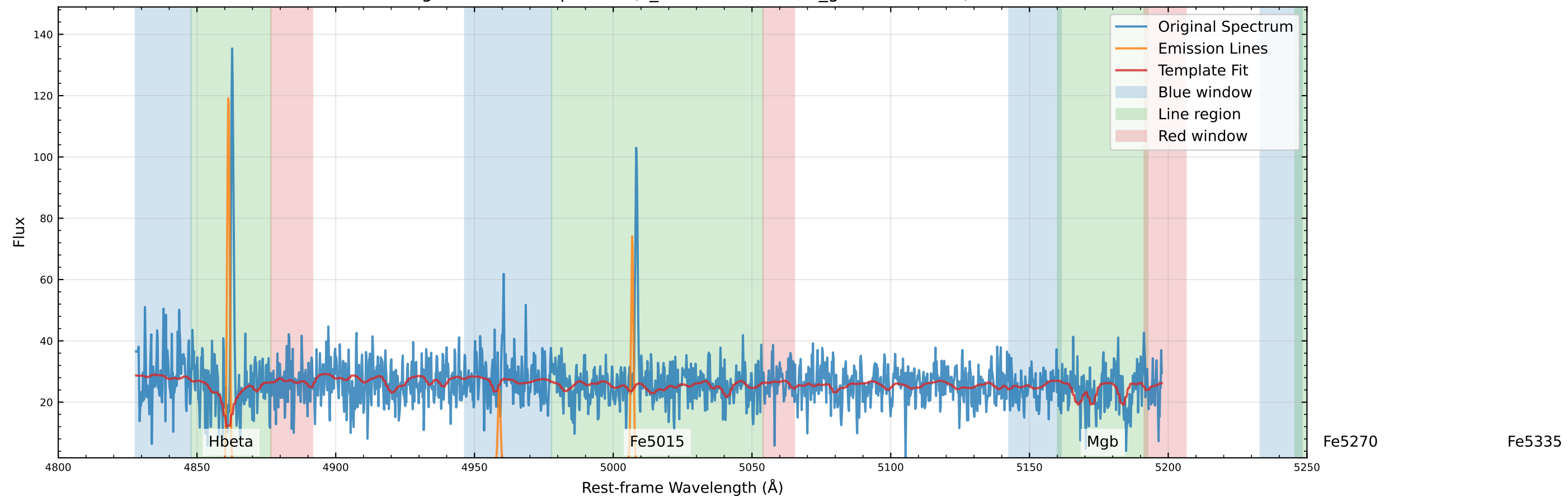
Original Data Comparison (v_star=86.4 km/s, v_gas=86.7 km/s)
