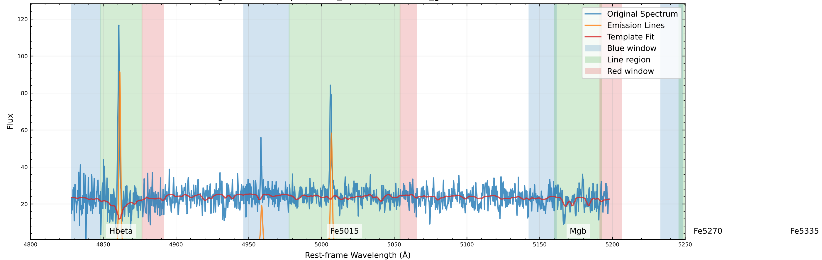
Original Data Comparison (v_star=-51.4 km/s, v_gas=-40.2 km/s)
