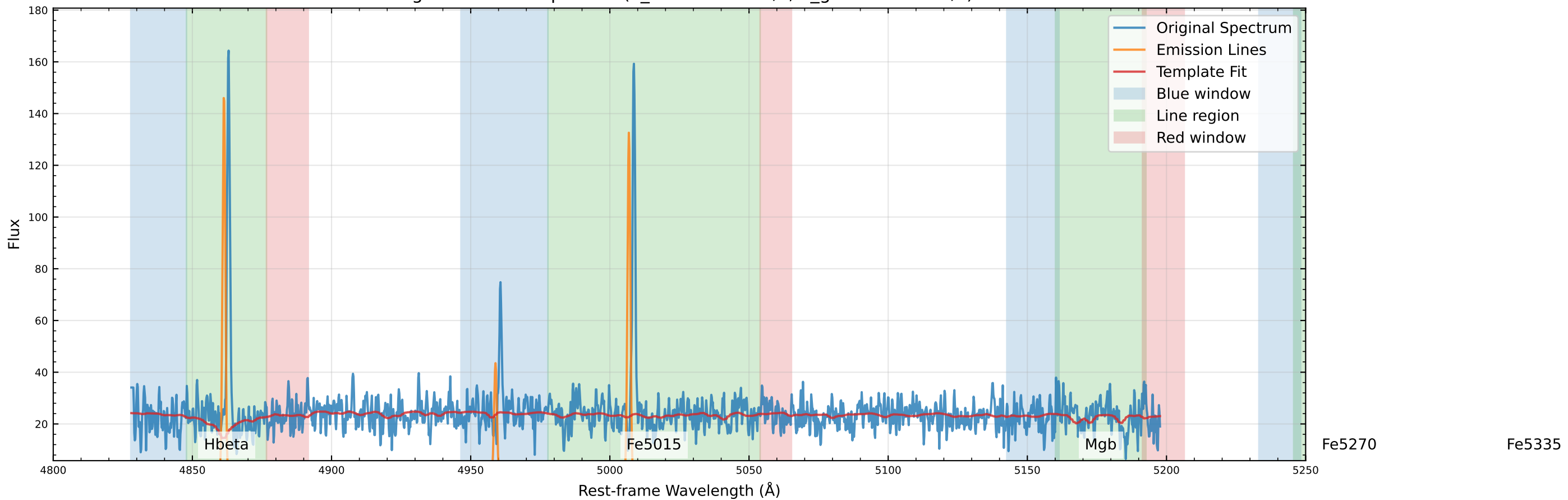
Original Data Comparison (v_star=99.9 km/s, v_gas=103.8 km/s)
