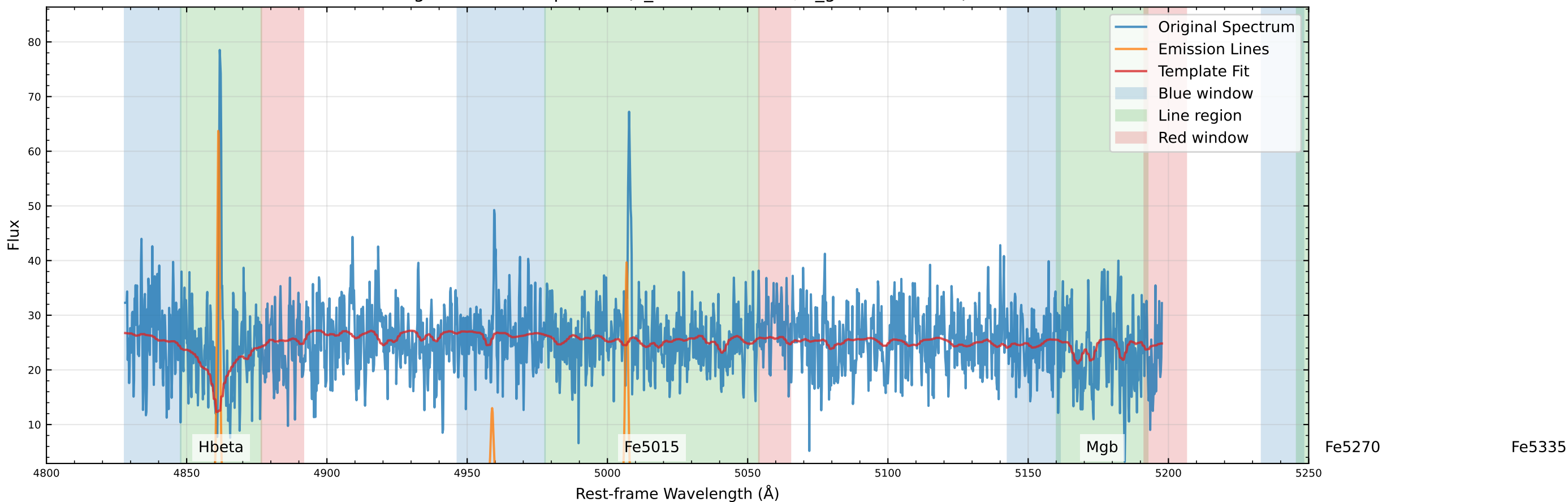
Original Data Comparison (v_star=45.3 km/s, v_gas=44.1 km/s)
