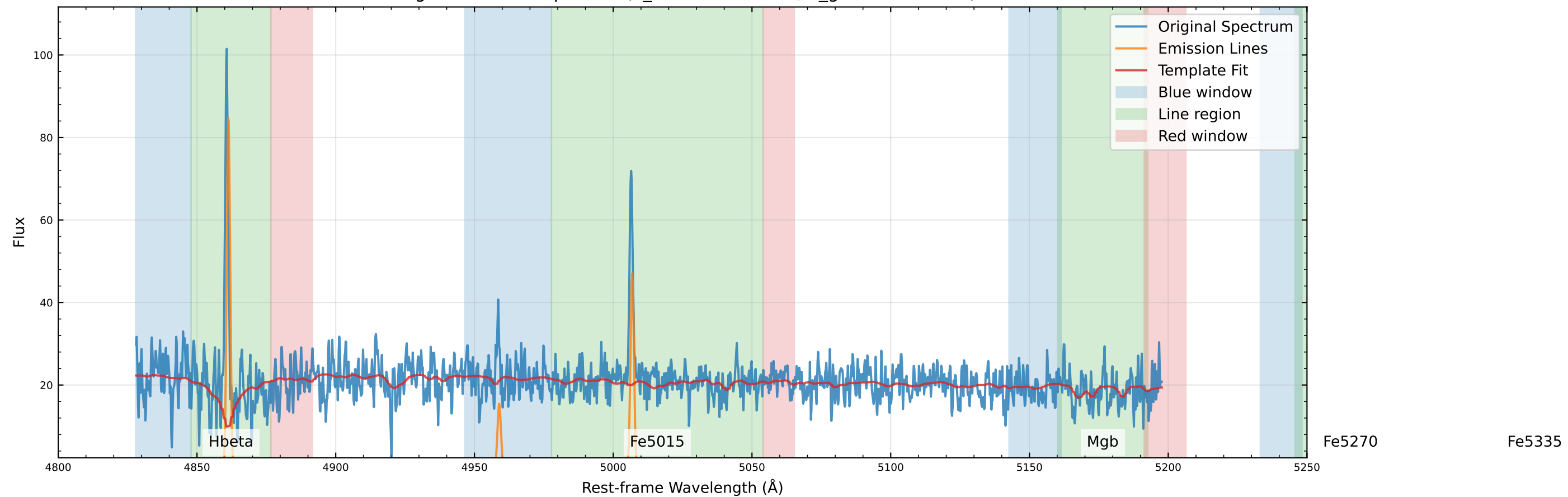
Original Data Comparison (v_star=-56.0 km/s, v_gas=-35.7 km/s)
