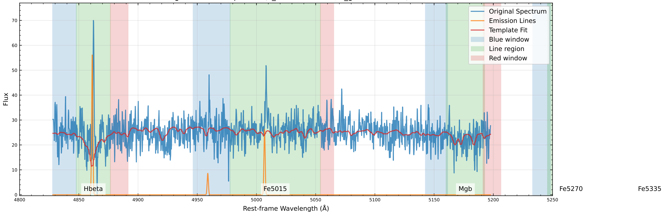
Original Data Comparison (v_star=75.1 km/s, v_gas=67.7 km/s)
