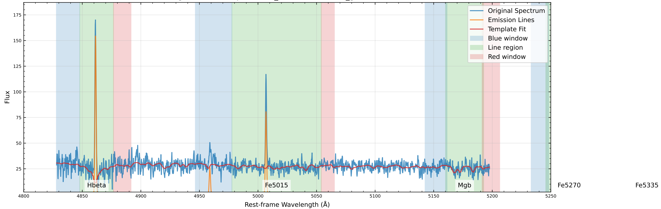
Original Data Comparison (v_star=11.1 km/s, v_gas=-3.1 km/s)
