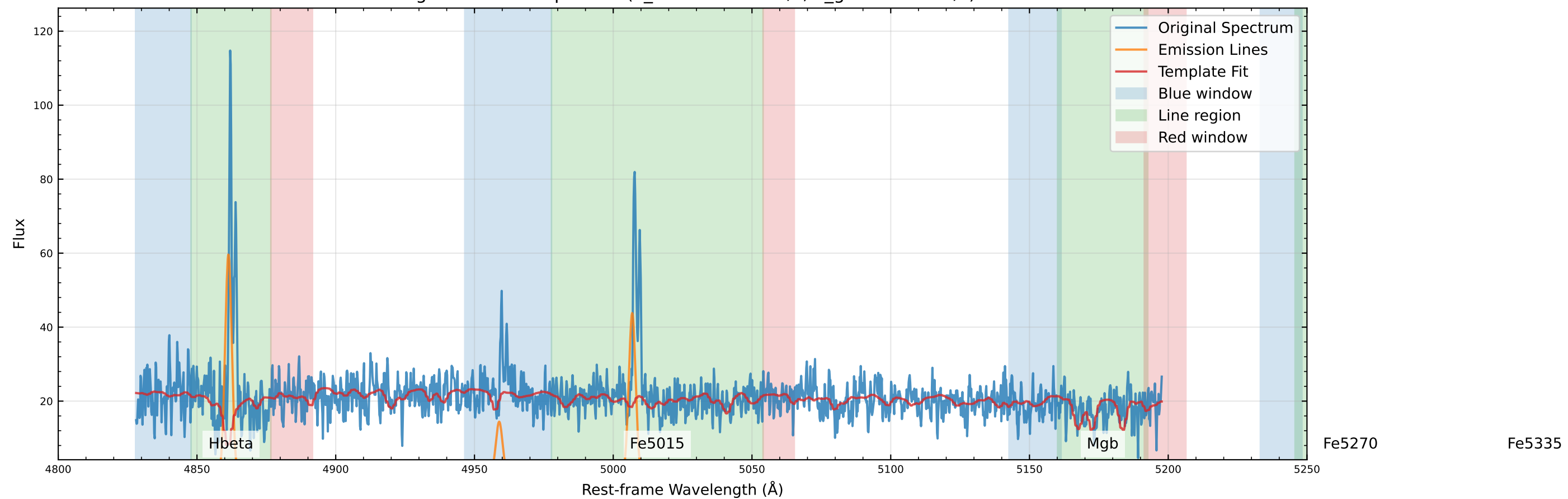
Original Data Comparison (v_star=113.2 km/s, v_gas=77.1 km/s)
