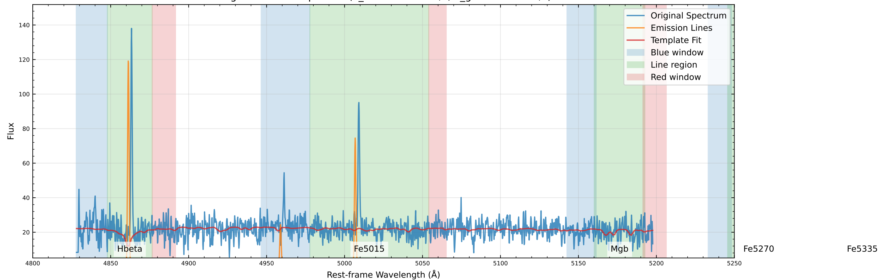
Original Data Comparison (v_star=146.9 km/s, v_gas=129.5 km/s)
