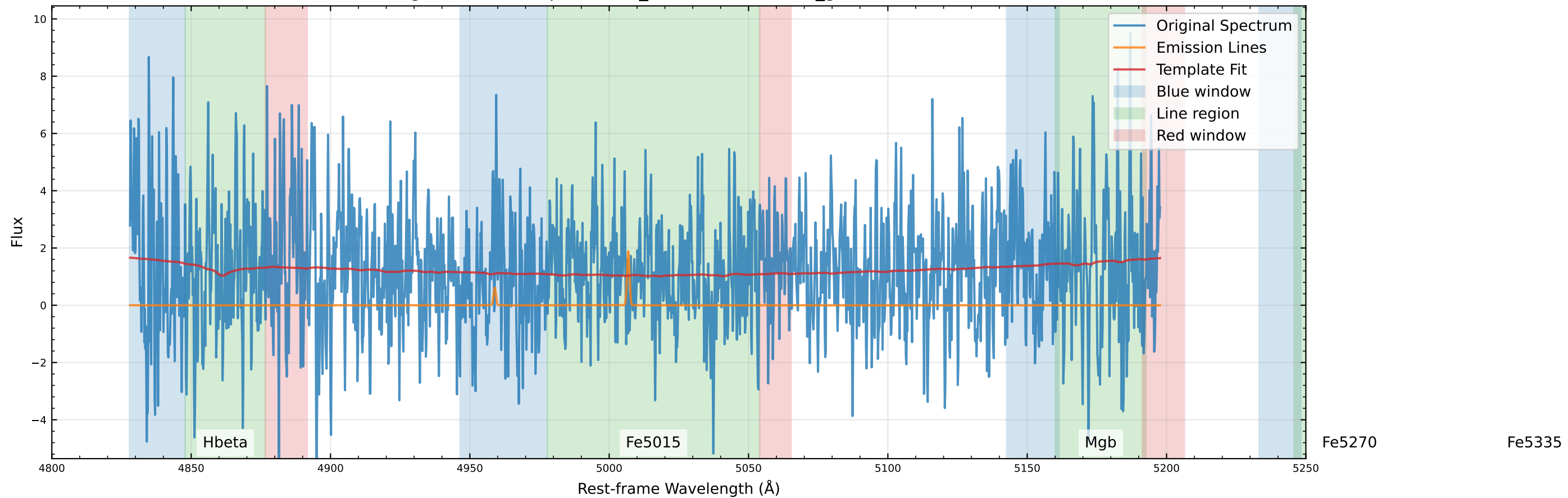
Original Data Comparison (v_star=-71.1 km/s, v_gas=-86.9 km/s)
