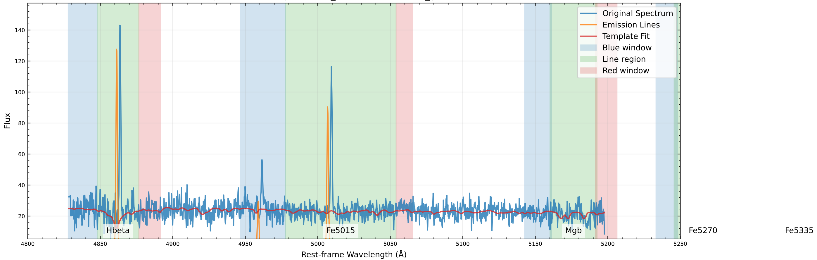
Original Data Comparison (v_star=168.8 km/s, v_gas=149.0 km/s)
