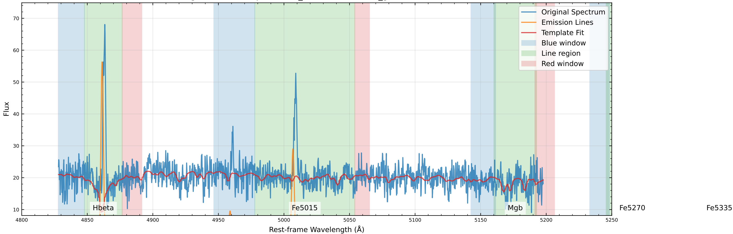
Original Data Comparison (v_star=88.3 km/s, v_gas=104.9 km/s)
