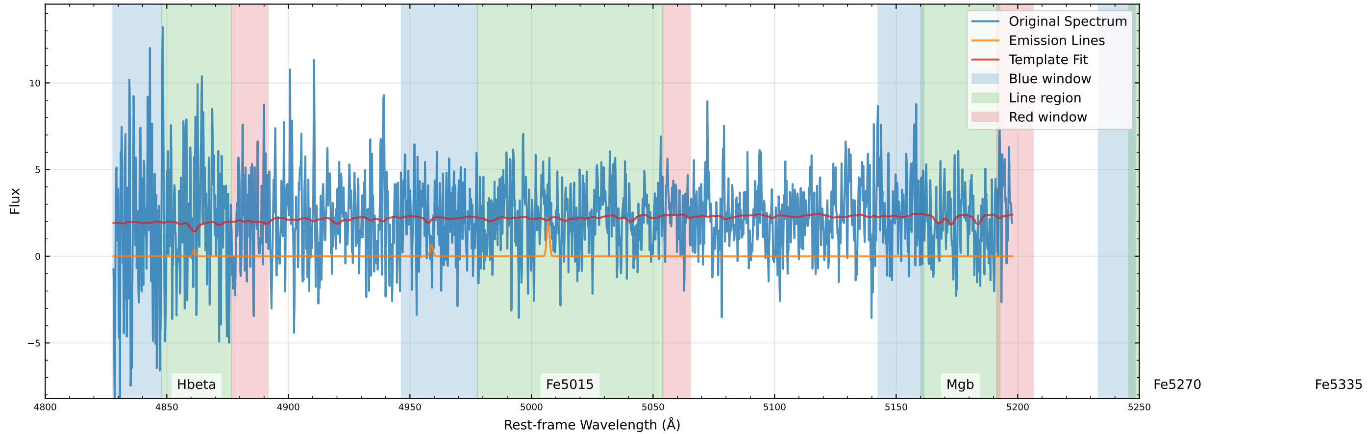
Original Data Comparison (v_star=-131.2 km/s, v_gas=-131.9 km/s)
