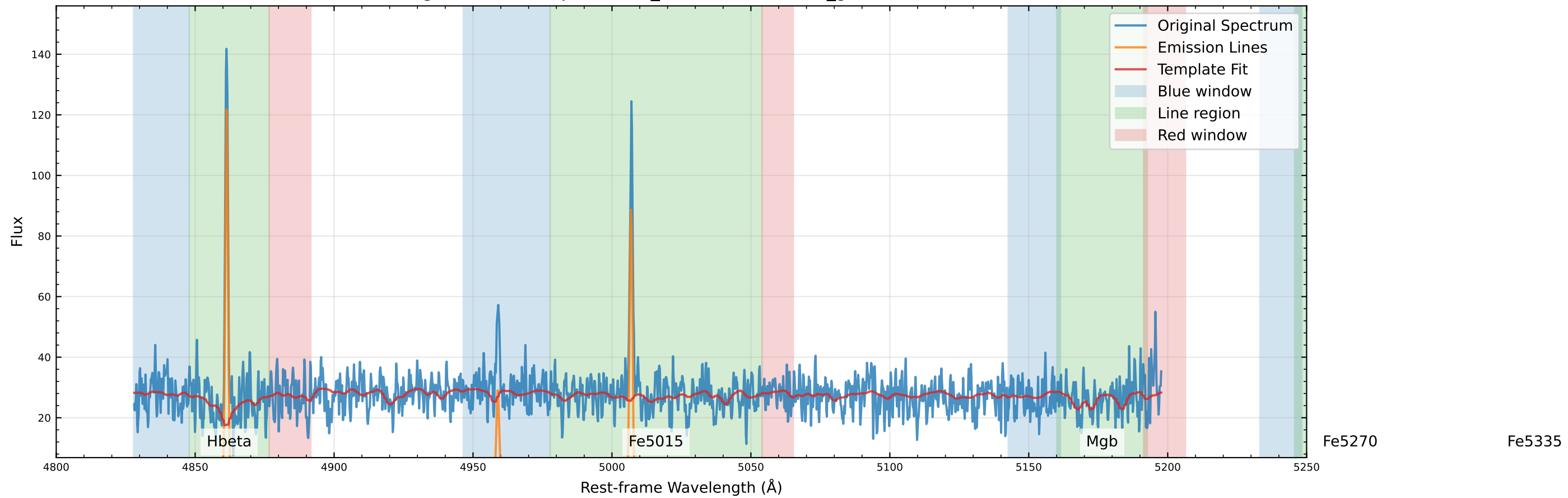
Original Data Comparison (v_star=-11.0 km/s, v_gas=2.2 km/s)
