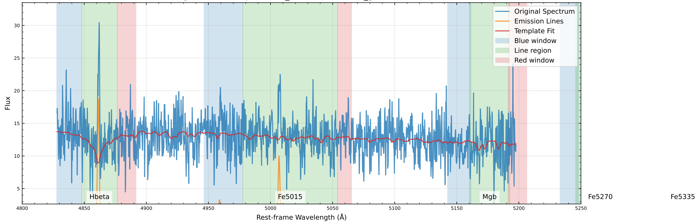
Original Data Comparison (v_star=-34.4 km/s, v_gas=21.6 km/s)
