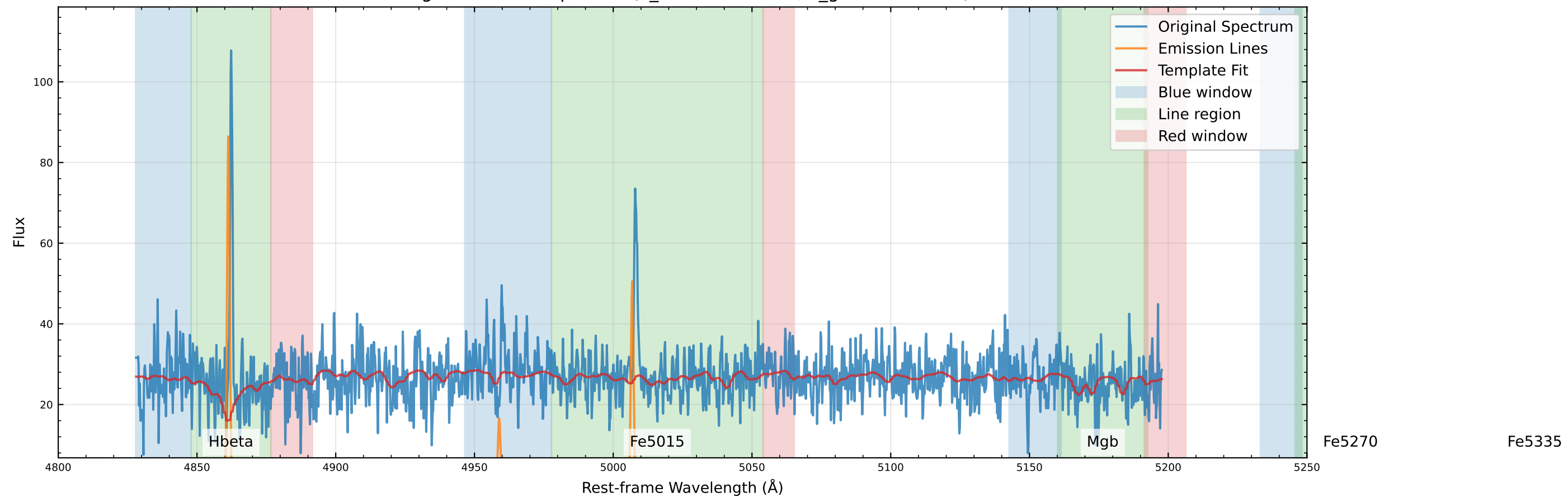
Original Data Comparison (v_star=83.5 km/s, v_gas=66.4 km/s)
