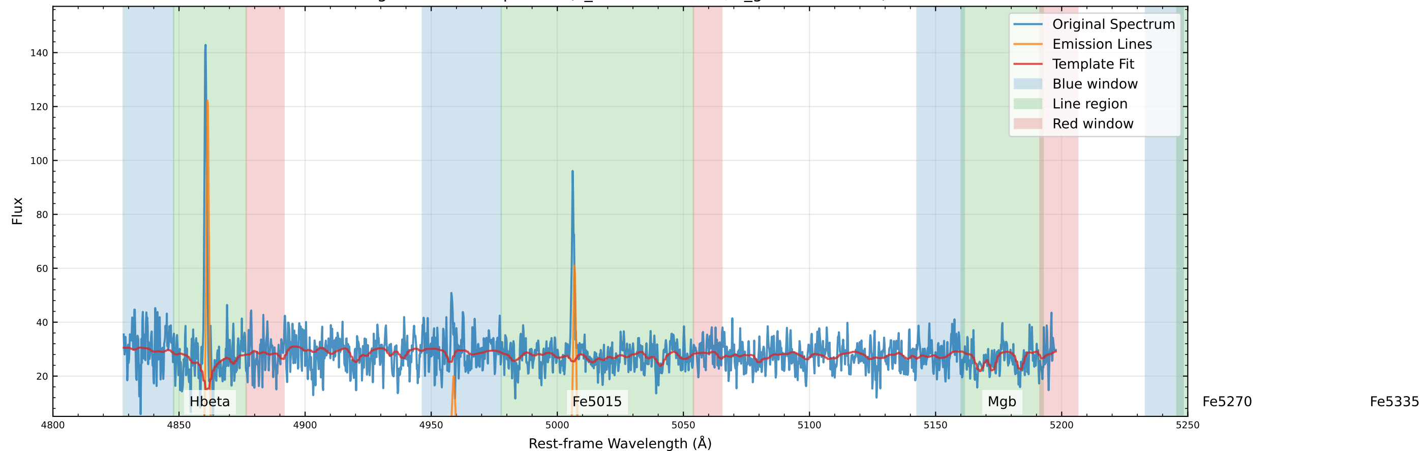
Original Data Comparison (v_star=-69.8 km/s, v_gas=-46.7 km/s)
