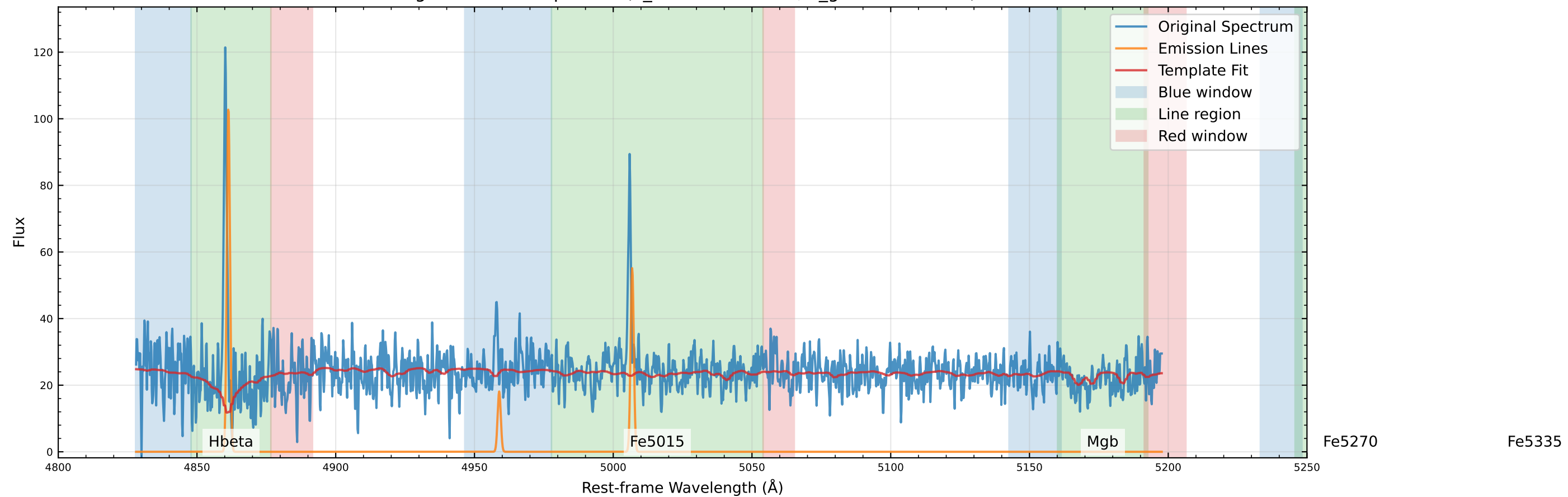
Original Data Comparison (v_star=-76.1 km/s, v_gas=-67.0 km/s)
