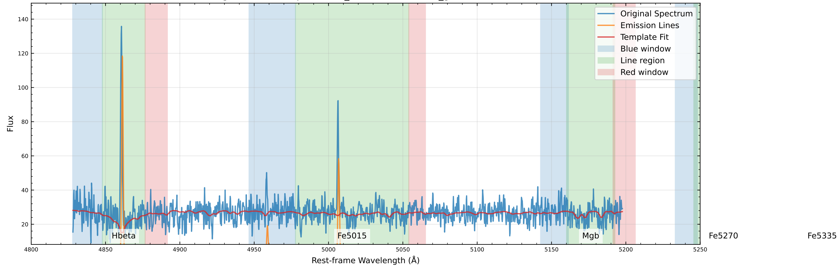
Original Data Comparison (v_star=-37.2 km/s, v_gas=-39.9 km/s)
